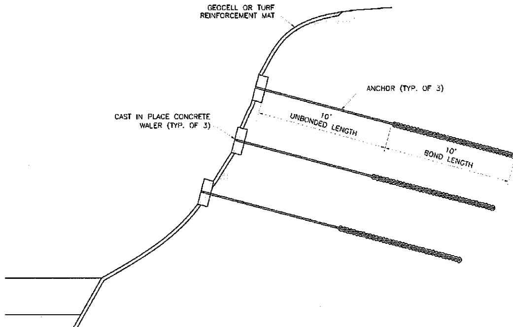
Figure 3.2 – Waler and Anchor System: Typical Section
