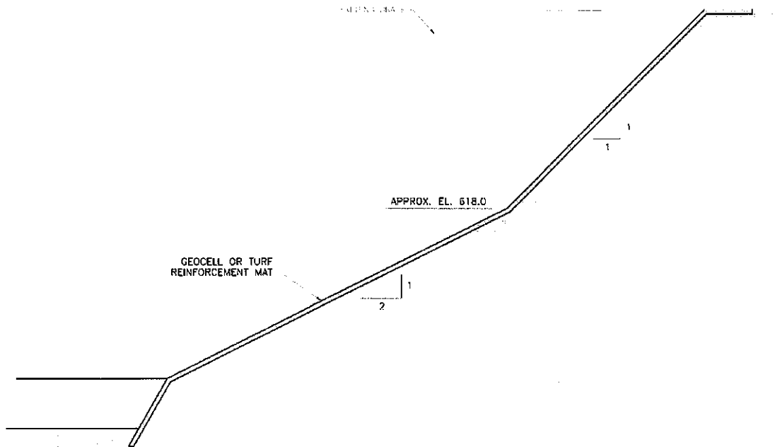
Figure 3.1 – Slope Reducing Alternative: Typical Section
